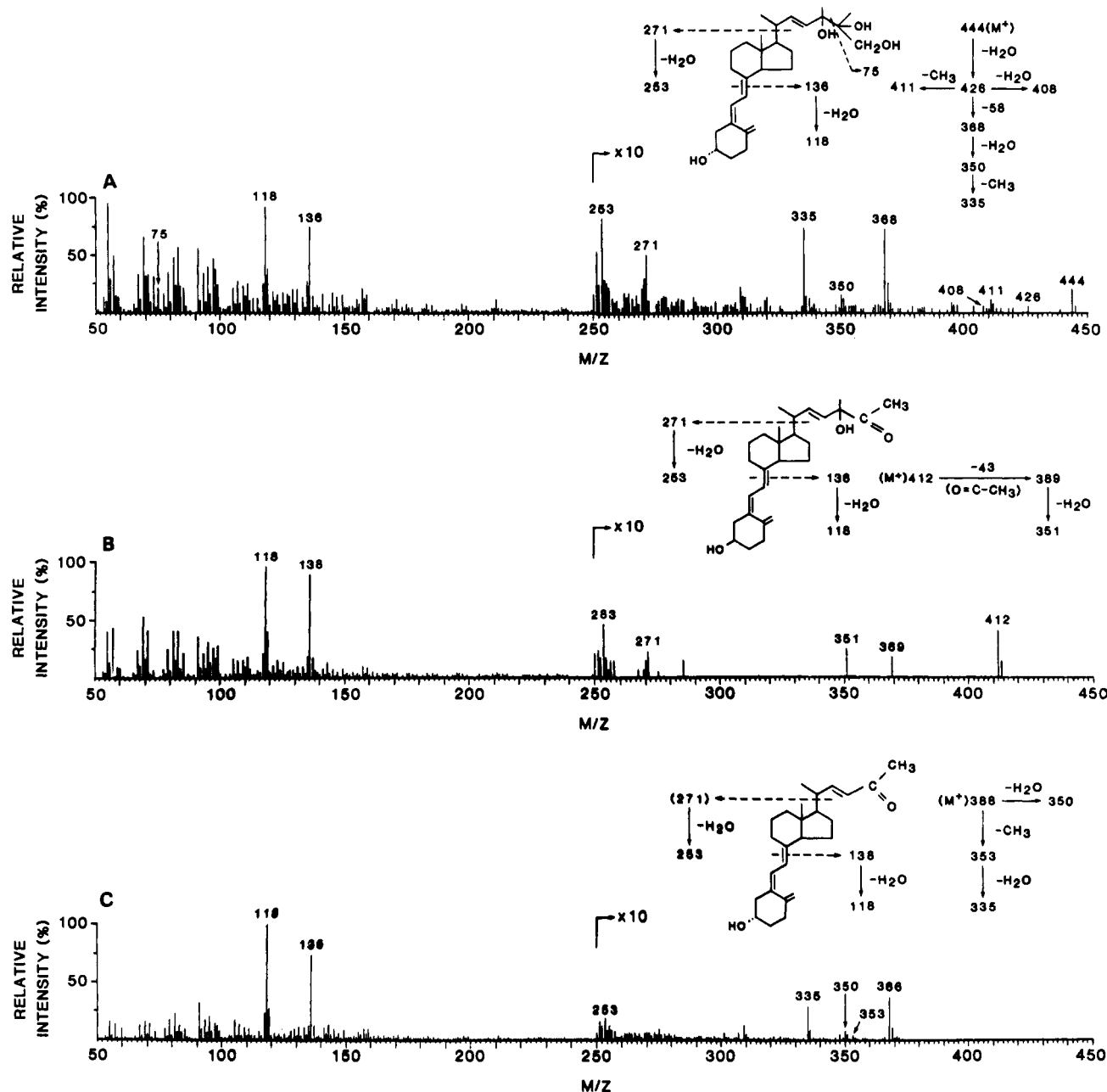
FIGURE 4: Mass spectra of 24,25,26(OH) 3 D 2 (A) and its two periodate cleavage products (B and C).
