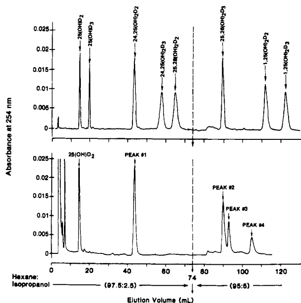
FIGURE 1: HPLC profiles of a mixture of various authentic synthetic metabolites of vitamins D 2 and D 3 (upper panel) and the lipid extract obtained from 20 mL of perfusate (lower panel): HPLC in both cases was performed on a Zorbax-Sil column (25 cm × 4.6 mm) that was first eluted with hexane–2-propanol (97.5:2.5) at a flow rate of 2 mL/min until 25,28(OH) 2 D 2 was eluted out of the column. Then, the first solvent system was changed to a second solvent system (hexane–2-propanol, 95:5), keeping the flow rate same to elute the more polar metabolites of vitamin D 2 out of the column. The various metabolites of 25-OH-D 2 were identified by monitoring their UV absorbance at 254 nm. Peaks 1, 2, and 4 represent 24,25(OH) 2 D 2 , 24,25,28(OH) 3 D 2 , and 24,25,26(OH) 3 D 2 , respectively. Peak 3 represents a non vitamin D contaminant produced by the kidney. Note that the size of the 25-OH-D 2 peak shown in the lower panel of the figure represents only 1/10 that of the original peak.
