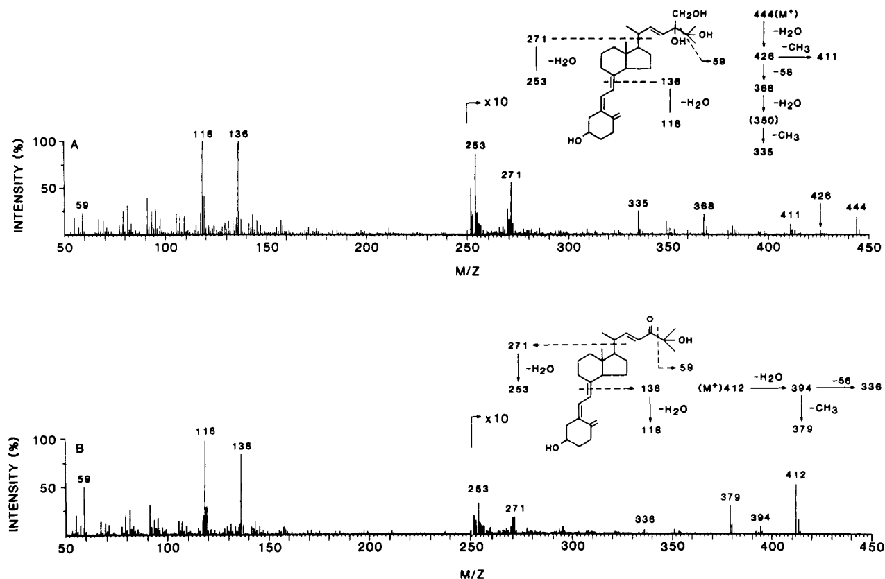
FIGURE 3: Mass spectra of 24,25,28(OH) 3 D 2 (A) and its periodate cleavage product (B).
