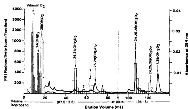
FIGURE 5: HPLC profile of the lipid extract of a plasma sample (3 mL) obtained from a rat given 1000 \mu\text{g} of [ ^3\text{H} ]vitamin \text{D}_2 in divided doses over a period of 10 days. The plasma sample was mixed with authentic nonradioactive vitamin \text{D}_2 metabolites [24-OH- \text{D}_2 , 0.2 \mu\text{g} ; 25-OH- \text{D}_2 , 0.2 \mu\text{g} ; 25,28(OH) _2\text{D}_2 , 0.2 \mu\text{g} ; 24,25,28(OH) _3\text{D}_2 , 0.5 \mu\text{g} ; 1,25(OH) _2\text{D}_2 , 0.5 \mu\text{g} ] with the aim of identifying each individual radioactive vitamin \text{D}_2 metabolite by its comigration with its corresponding authentic nonradioactive vitamin \text{D}_2 metabolite standard. The lipid extract of the plasma sample containing the various [ ^3\text{H} ]vitamin \text{D}_2 metabolites and the authentic nonradioactive vitamin \text{D}_2 metabolites was analyzed by HPLC under the chromatographic conditions described in the legend to Figure 1 except that the first solvent system was changed to the second solvent system at an elution volume of 90 mL. The elution positions of the various nonradioactive authentic standards of vitamin \text{D}_2 metabolites as monitored by their UV absorbance at 254 nm are depicted in the figure above by the solid line. Note that the UV absorbance profile during the first 10-min HPLC run is not shown for the sake of clarity. Fractions of 1 mL during the first 10 min of the HPLC run and fractions of 2 mL during the remaining period of the HPLC run were collected. The HPLC effluent in each fraction was divided into two equal portions. The first portion was used to measure the radioactivity, which is depicted in the figure by a histogram. The second portion was used for rechromatography of each major metabolite of vitamin \text{D}_2 on a second HPLC run using a methylene chloride–2-propanol mixture as the solvent system (data not shown). Thus, we confirmed the identity of each major metabolite of vitamin \text{D}_2 by its comigration with its corresponding authentic cold standard on two different HPLC systems.
